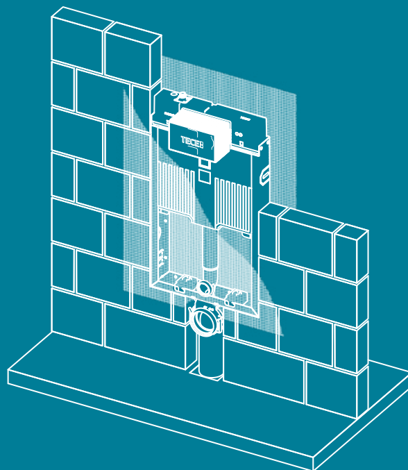
Installation in a masonry pre-wall
