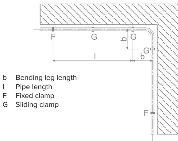
Compensation of thermal linear extension in a direction change
